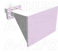
LB-187-15-C-NFSPO Standard Gain Horn Antenna 3.95-5.85GHz 15dB Gain N Type Female
