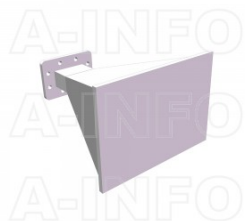
LB-187-15-ASPO Standard Gain Horn Antenna 3.95-5.85GHz 15dB Gain Rectangular Waveguide Interface
